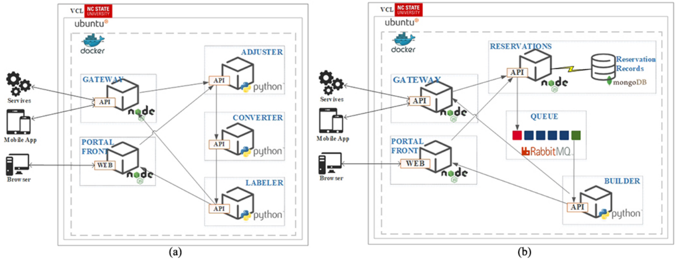
Fig. 2. Testbed a) Case Study 2, b) Case Study 3
